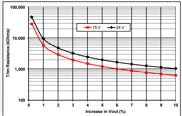
Common Figure 4: Trim graph for trim-up 15 to 24 V outputs.
