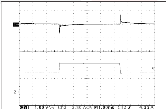
Figure 5: Output voltage response to step-change in load current (50%-75%-50% of Iout(max); di/dt = 0.1A/\mu s ). Load cap: 15 \mu F tantalum cap and 1 \mu F ceramic cap. Ch 1: Vout, Ch 2: Iout.
